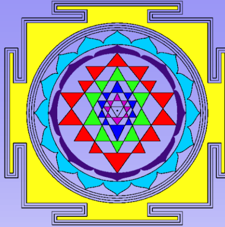
Sri Yantra
