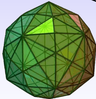
Disdyakis Triacontahedron
