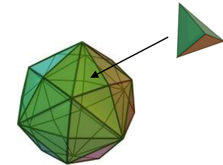
Disdyakis dodecahedron
