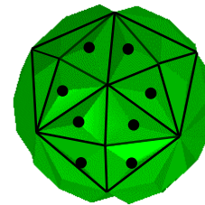
144 Polyhedron
