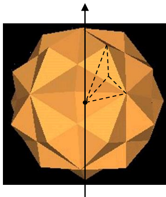
disdyakis triacontahedron
