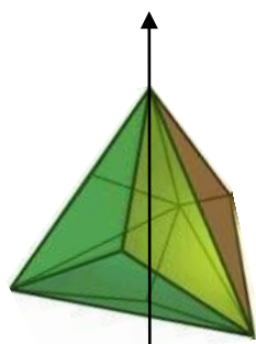
triakis tetrahedron
