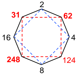
Figure 10a. The eight non-trivial factors of 496 , the dimension of the superstring gauge symmetry groups O(32) and E_8 \times E_8 , can be divided into two geometric sequences of four integers that double in size.
