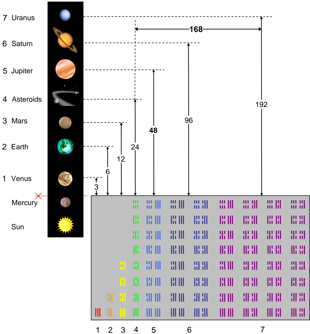
Figure 26. The Titius-Bode distances from the asymptotic centre (shown as X) of the seven planets in the first octet after Mercury are the numbers of yin/yang lines in the seven successive doublings of sets of trigrams.
