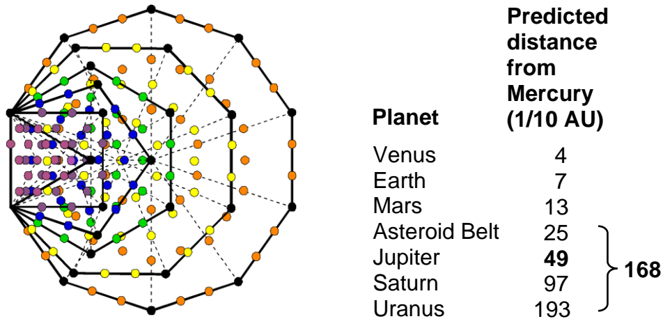
Figure 27. Associated with each set of six polygons in the inner form of the Tree of Life are 25 (●) corners and 168 coloured yods. They denote the predicted distance 25 (in units of 1/10 AU) between Mercury and the Asteroid Belt and the distance 168 between the Asteroid Belt and Uranus.
